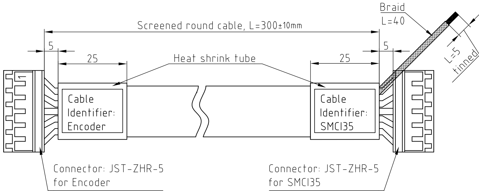
PIN ASSIGNMENT JST-ZHR-5 FOR ENCODER
